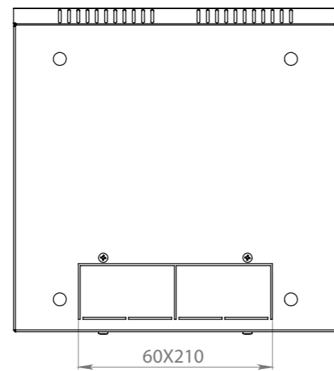
BOTTOM VIEW
